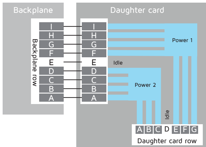
Power wafer to backplane pin mapping
